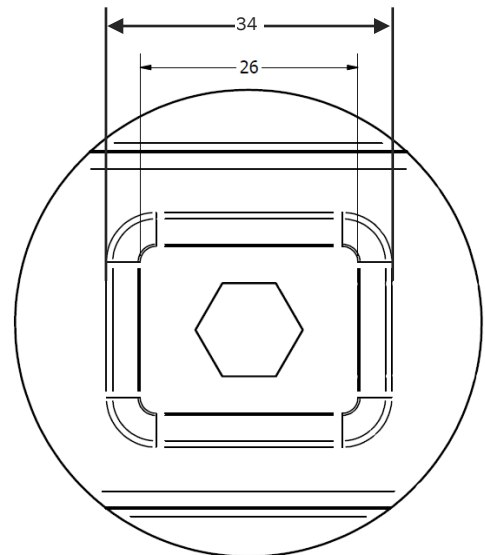
Figure 5: Rivet Nut hole dimensions
