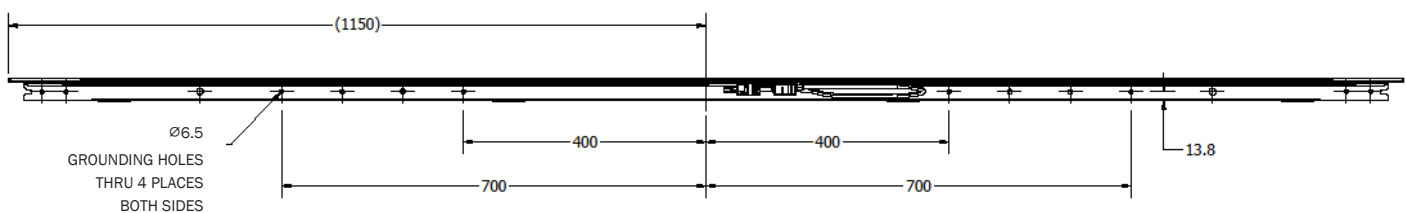
Figure 12: Grounding hole size and locations
