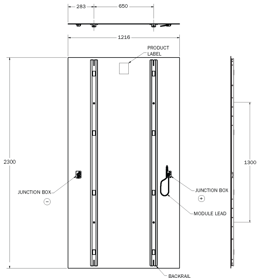
Figure 3: Series 7 FT1 Module Mechanical Drawing. All dimensions are in mm.
