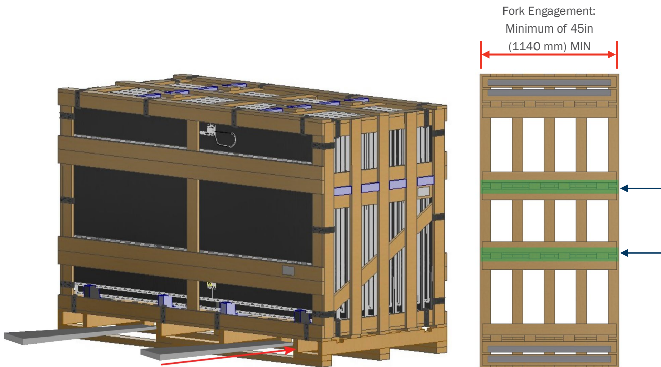
Figure 2: Series 7 FT1 Long Side Forklift Engagement
