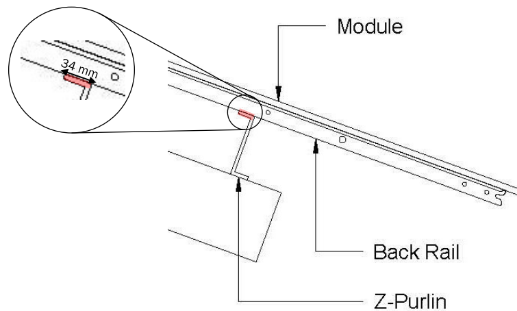
Figure 7: Mounting Structure Z-Purlin Minimum Width
