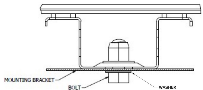
Figure 6: Rivet Nut mounting details
