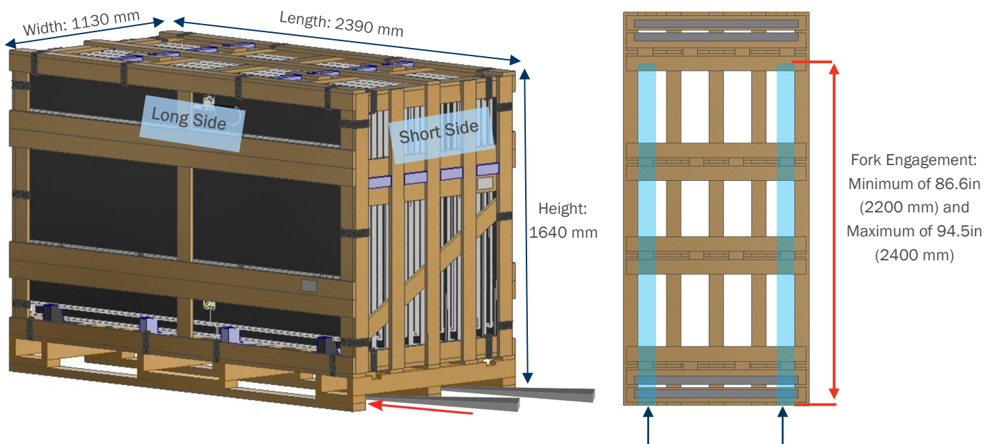
Figure 1: Series 7 FT1 Short Side Forklift Engagement
