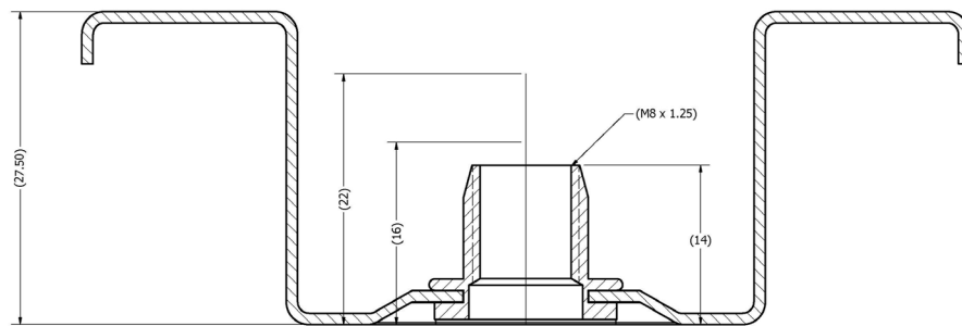
Figure 4: Cross sectional View of Module Back Rail
